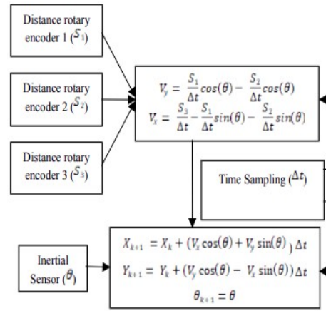
Fig. 2. Block Diagram Forward Kinematic [3]
