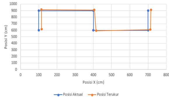
Fig. 8. Robot Estimate Position Graph
